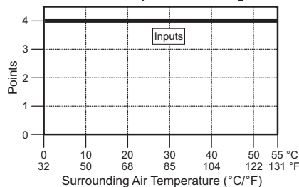
C0-02DD1-D Temperature Derating Chart
