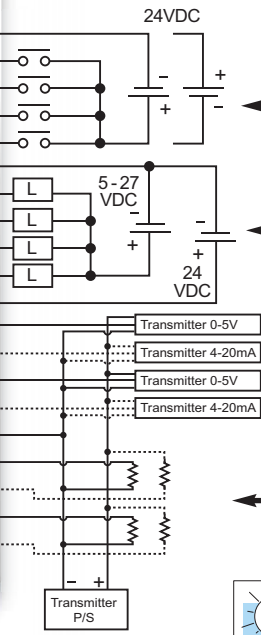
Wiring Diagram
