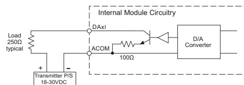
Analog Current Output Circuit
