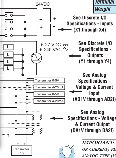
Wiring Diagram
